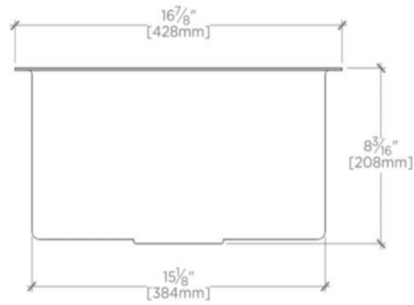
FRONT VIEW SCALE: 1\frac{1}{2}"=1'-0"
